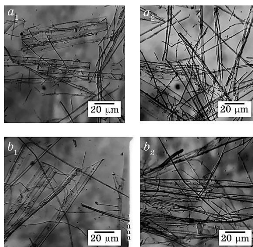
Fig. 3. Microphotographs of polypropylene residues after extraction of the matrix component from the extrudates of mixtures: a ) the original PP/PVA 2 ( a 1 —films, a 2 —microfibrils); b ) PP/PVA 2 /CNTs with a content of 0.5 wt.% CNTs ( b 1 —films, b 2 —microfibrils).
