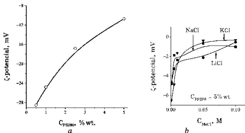
Fig. 1. Zeta potential as a function of PS200 concentration in electrolyte-free aqueous suspension (a) and in the presence of electrolytes (b): ●—LiCl, ■—NaCl, or ▼—KCl (in solution at C_{PS200} = 5 \text{ wt.}\% ).
