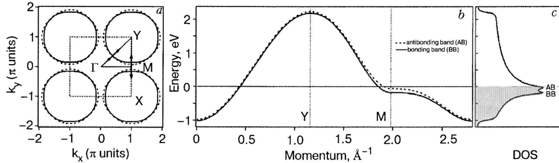
FIG. 4. The bare band dispersion, as extracted from experiment: 20 (a) Fermi surfaces, the dotted square denotes the boundary of the 1st BZ, the \Gamma YM triangle shows the path along which the dispersion is shown on panel (b); (c) the corresponding density of states (DOS) with two van Hove singularities close to E_F .
