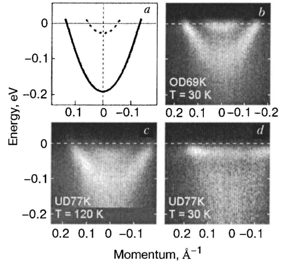
FIG. 2. Electronic structure in the antinodal region (along XMY cut). Bare band structure (a) and ARPES snapshots taken at 30 K (below T_c ) for an overdoped sample (OD, T_c = 69 K, x = 0.22 ) (b) and underdoped sample (UD, 77 K) (d), and for UD77 at 120 K (c). On panels (b) and (c) two split bands are well visible, while on panel (d) a strong depletion of the spectrum can be seen at some “mode” energy. 12
