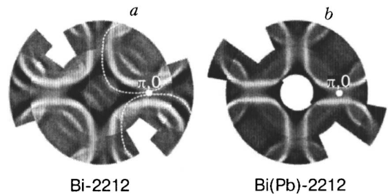
FIG. 3. Fermi surfaces measured on pristine Bi-2212 (a) and on superstructure-free lead-doped Bi(Pb)-2212 (b). 34
